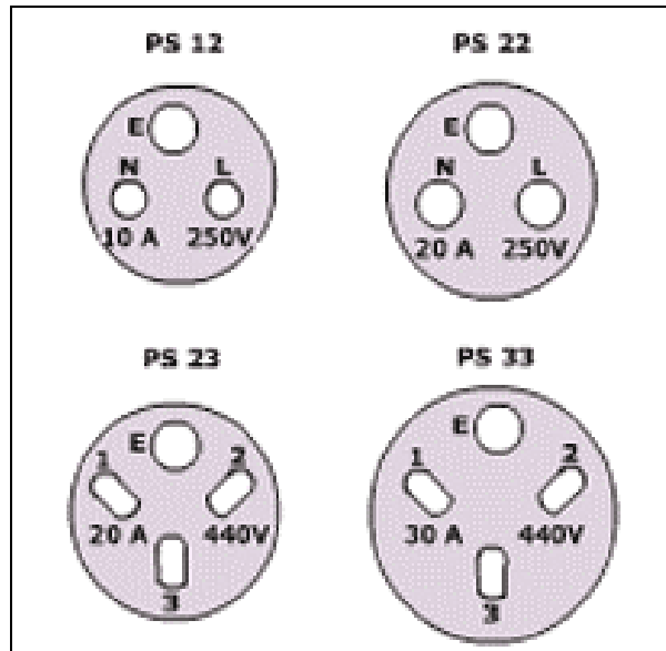
Typical Socket Interiors viewed from the front (Not to scale)
